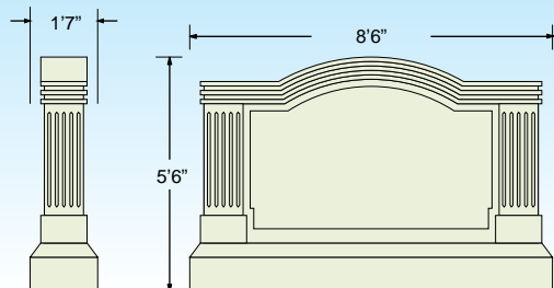
Square Columns
