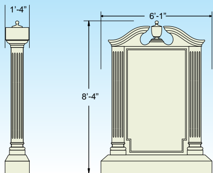
Square Columns
